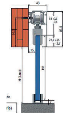
To wall
