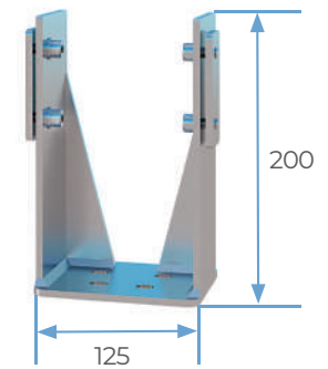
Adjustable Support
