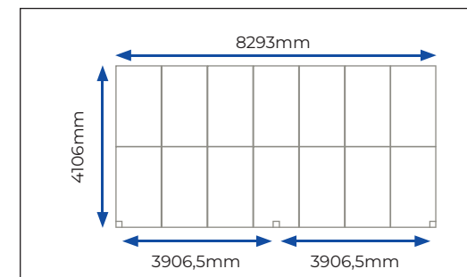
e-Orbita LUZ structure with gable roof
