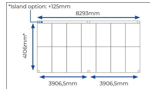
e-Orbita LUZ structure with wall configuration
