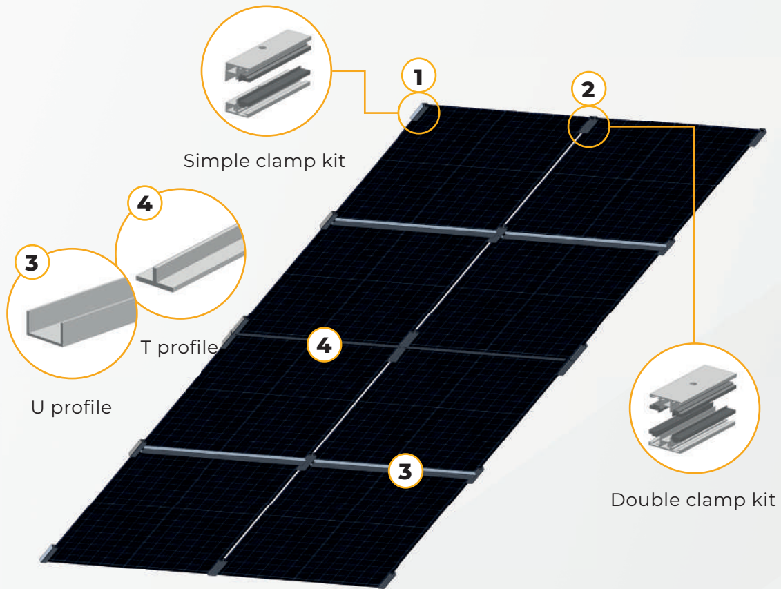
Ex. representation of the clamping of 4 glasses Suitable for all types of structures
