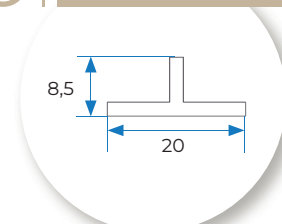
TRIMS UNDER PHOTOVOLTAIC GLASS
