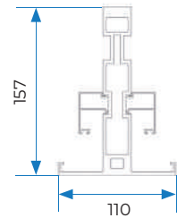
⑤ CENTRAL GUIDE
