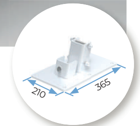
A - TYPE OF SUPPORT - Floor support
