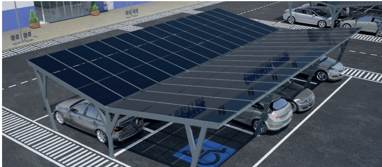
Example of an e-Orbita CAR solar carport in Y configuration (inverted gable roof)
