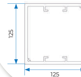
B1 CLOSED PILLAR PROFILE
