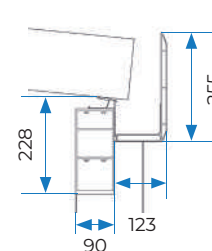
③ GUTTER + HEAVY BEAM
