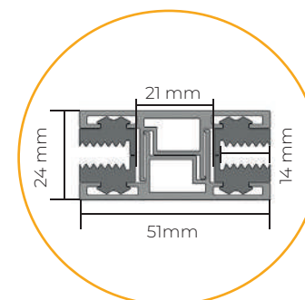
Double clamp kit
