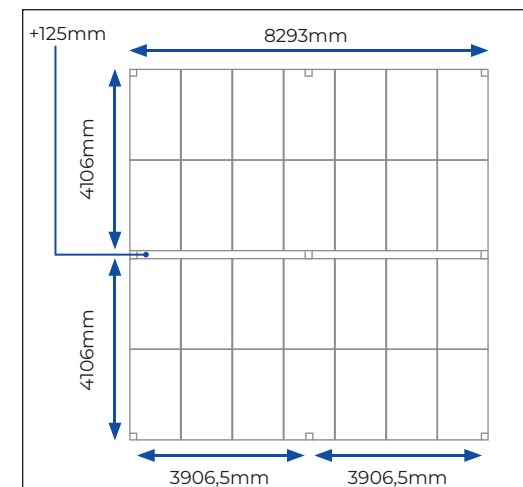
e-Orbita LUZ structure with gable roof
