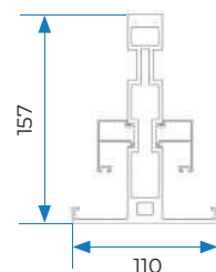
⑤ CENTRAL GUIDE
