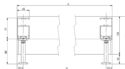
LINE SECTION
