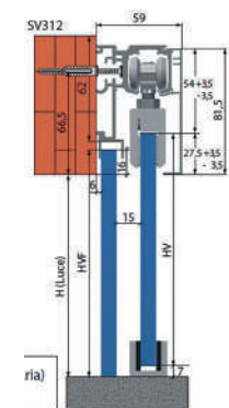
To wall
