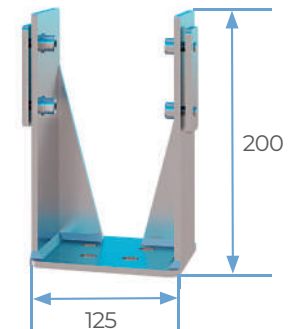
Adjustable support
